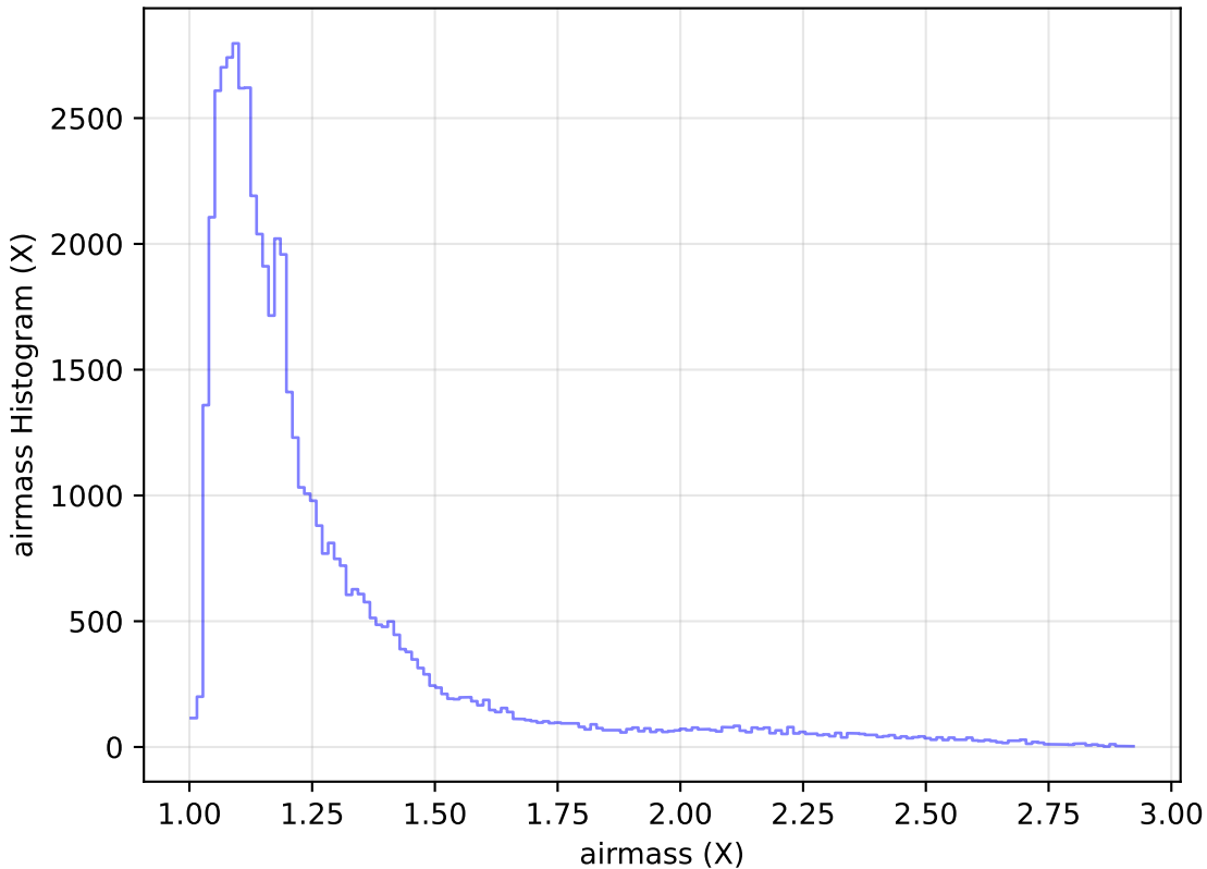
ddf_acor_sf15_lsf30_lsr10_v3.4_10yrs Yr 1 i band: airmass Histogram
