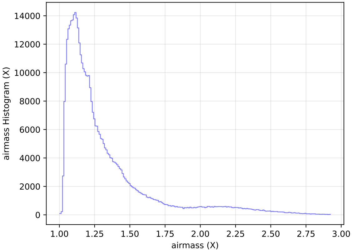
ddf_acor_sf15_lsf30_lsr10_v3.4_10yrs WFD z band: airmass Histogram
