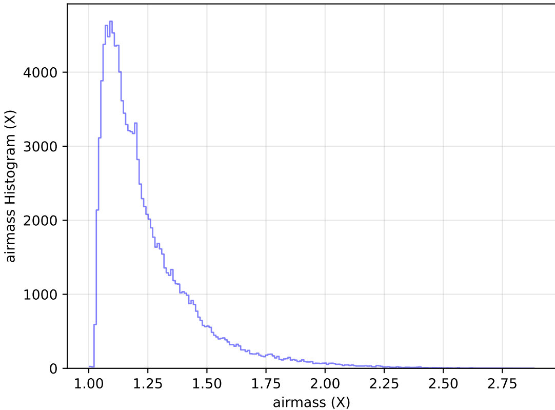
ddf_acor_sf15_lsf30_lsr10_v3.4_10yrs WFD u band: airmass Histogram
