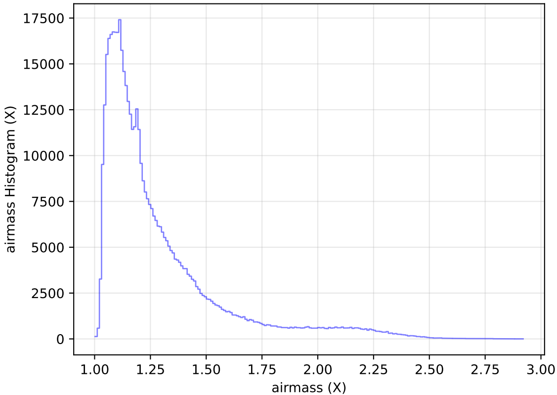
ddf_acor_sf15_Isf30_Isr10_v3.4_10yrs WFD r band: airmass Histogram
