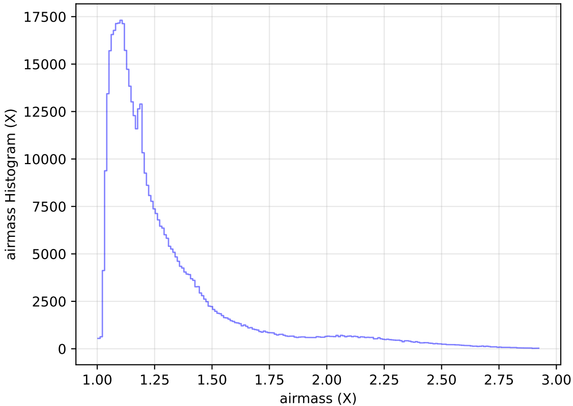
ddf_acor_sf15_lsf30_lsr10_v3.4_10yrs WFD i band: airmass Histogram
