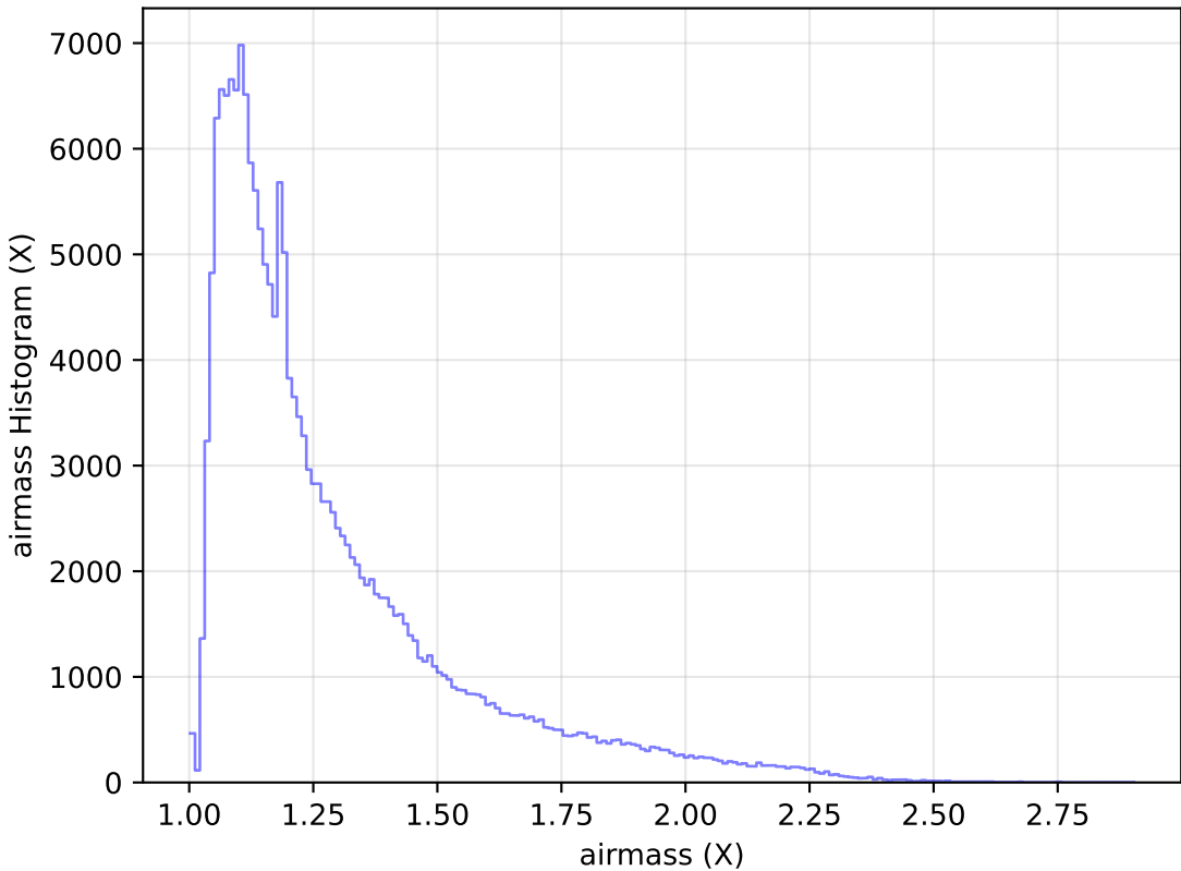
ddf_acor_sf15_lsf30_lsr10_v3.4_10yrs WFD g band: airmass Histogram
