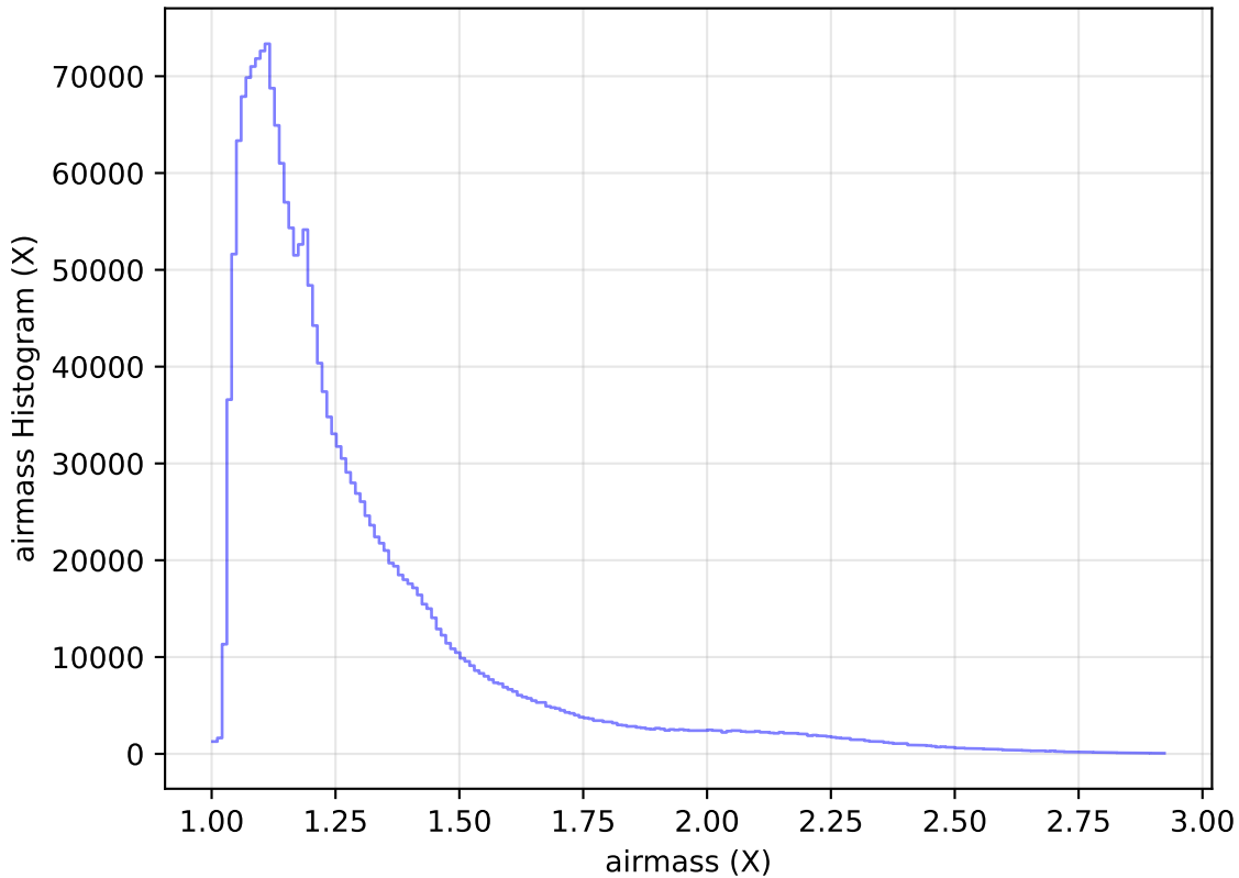
ddf_acor_sf15_lsf30_lsr10_v3.4_10yrs WFD all bands: airmass Histogram
