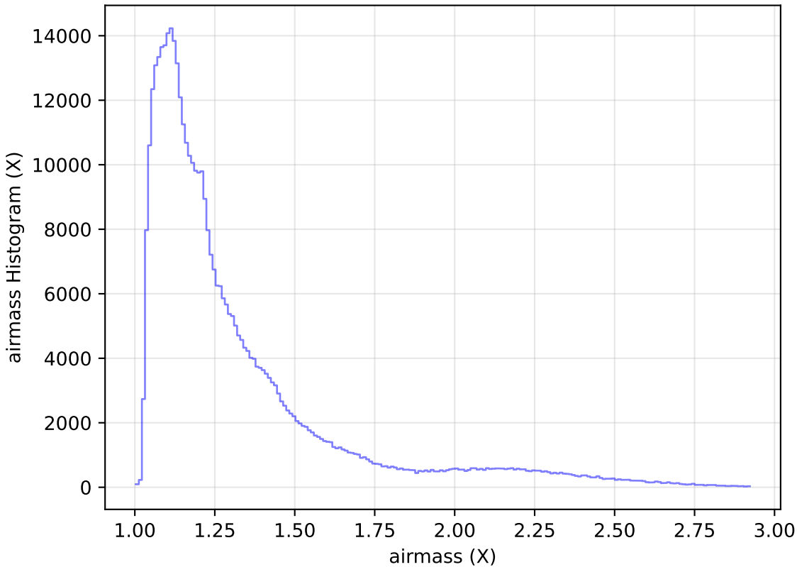
ddf_acor_sf15_lsf30_lsr10_v3.4_10yrs All sky z band: airmass Histogram
