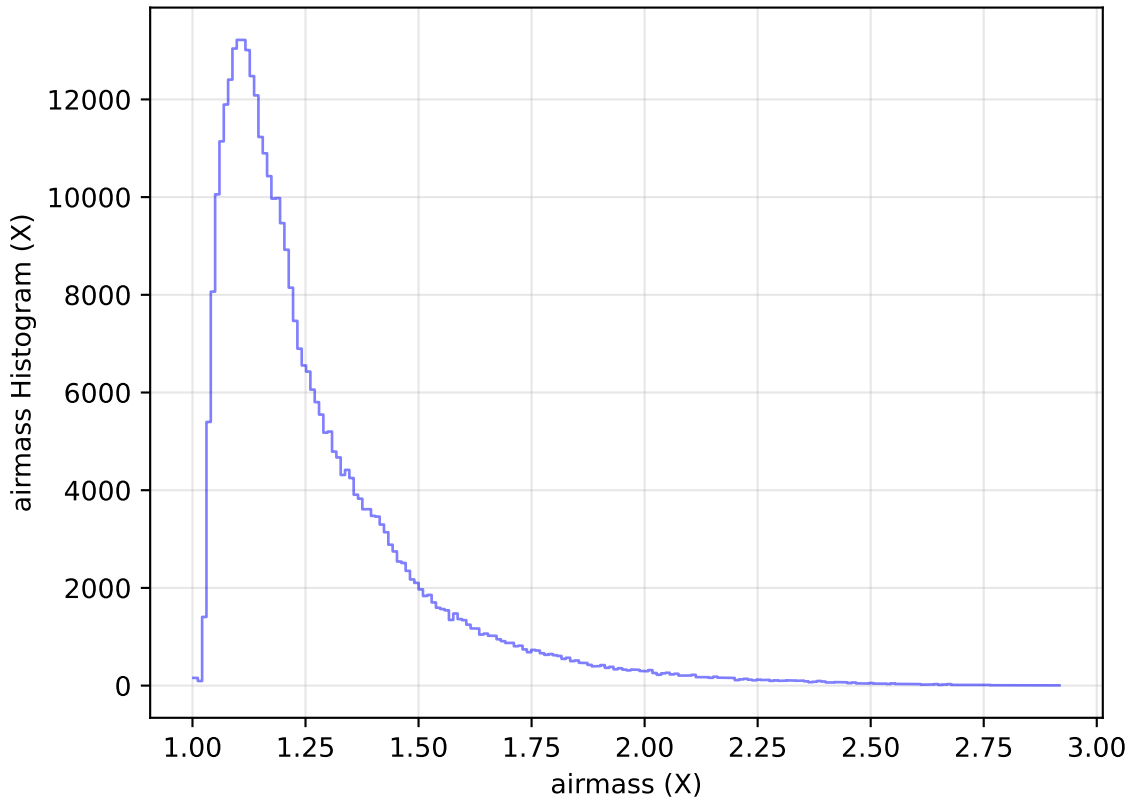
ddf_acor_sf15_lsf30_lsr10_v3.4_10yrs All sky y band: airmass Histogram
