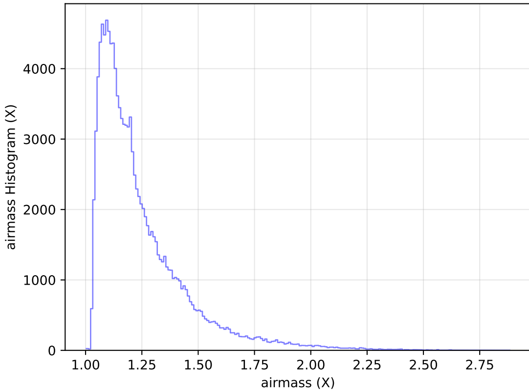
ddf_acor_sf15_lsf30_lsr10_v3.4_10yrs All sky u band: airmass Histogram
