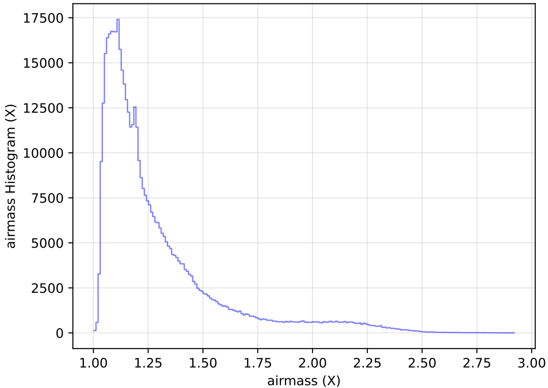
ddf_acor_sf15_lsf30_lsr10_v3.4_10yrs All sky r band: airmass Histogram
