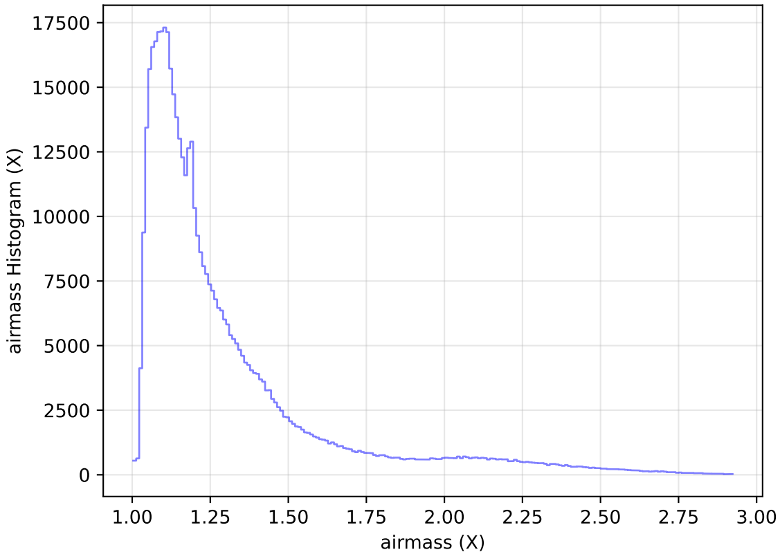
ddf_acor_sf15_lsf30_lsr10_v3.4_10yrs All sky i band: airmass Histogram
