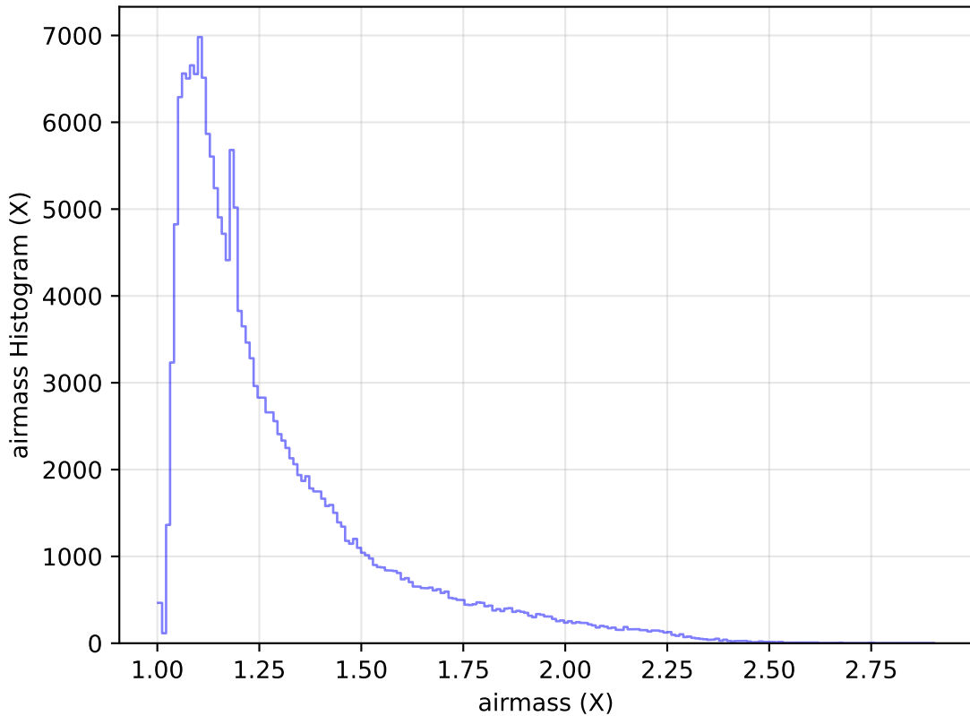
ddf_acor_sf15_lsf30_lsr10_v3.4_10yrs All sky g band: airmass Histogram
