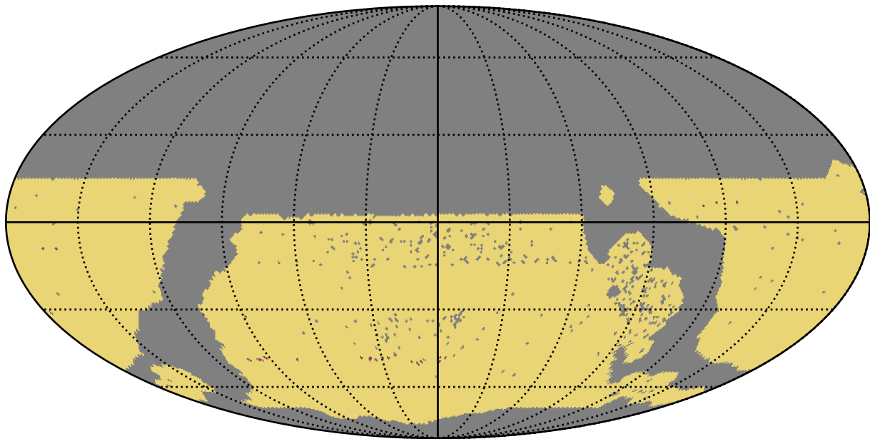
ddf_acor_sf15_lsf30_lsr10_v3.4_10yrs WFD: RapidRevisits
