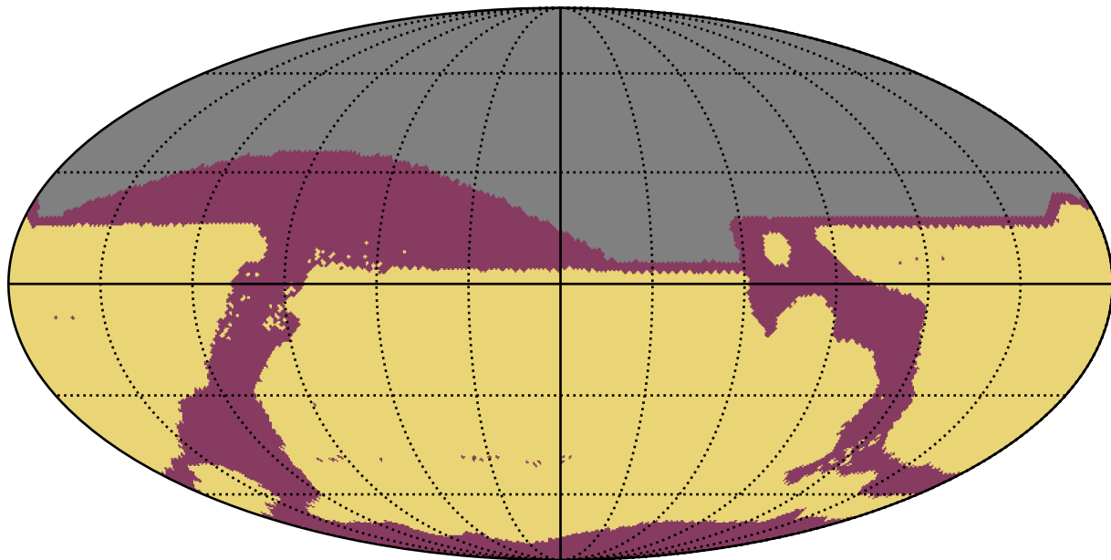
ddf_acor_sf15_lsf30_lsr10_v3.4_10yrs All sky: RapidRevisits
