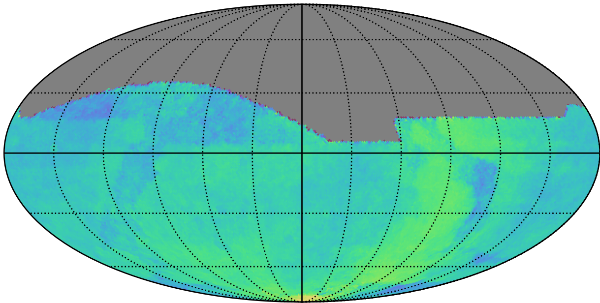
ddf_acor_sf15_lsf30_lsr10_v3.4_10yrs All sky: Parallax Coverage @ 22.4
