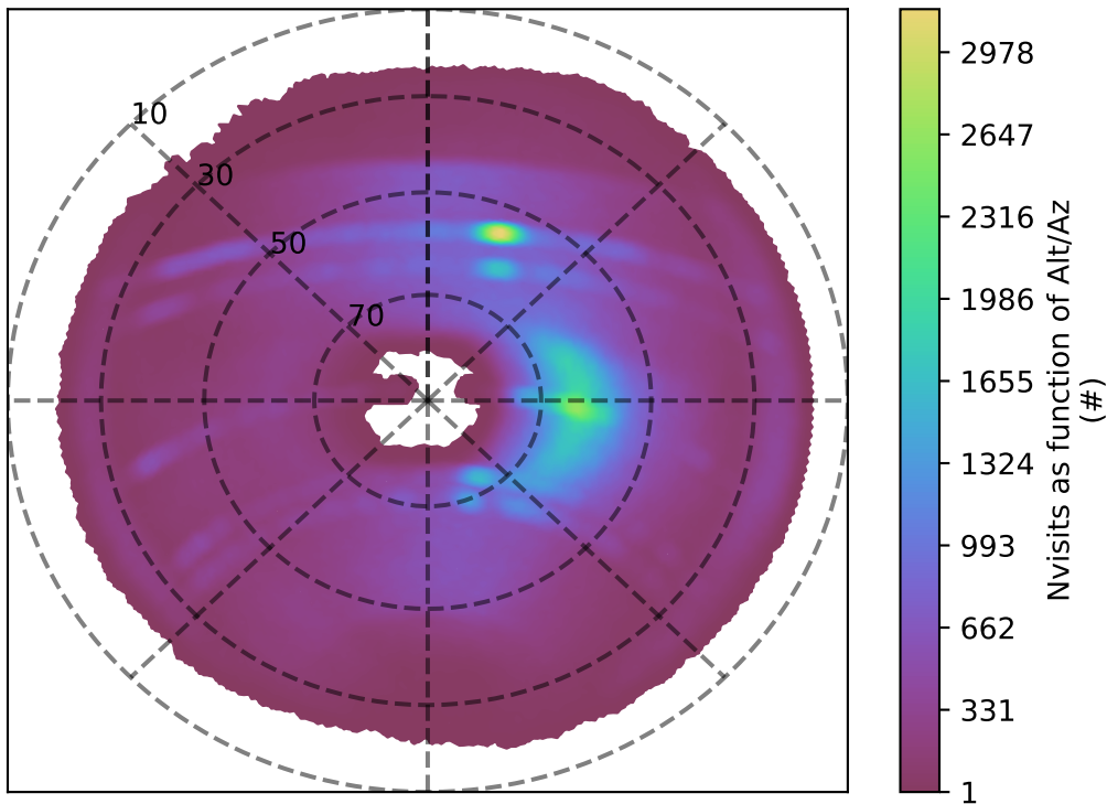
ddf_acor_sf15_lsf30_lsr10_v3.4_10yrs z band: Nvisits as function of Alt/Az
