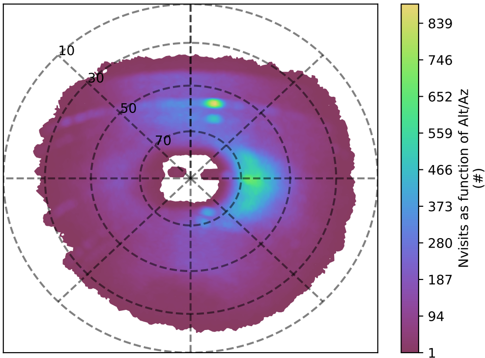
ddf_acor_sf15_lsf30_lsr10_v3.4_10yrs u band: Nvisits as function of Alt/Az
