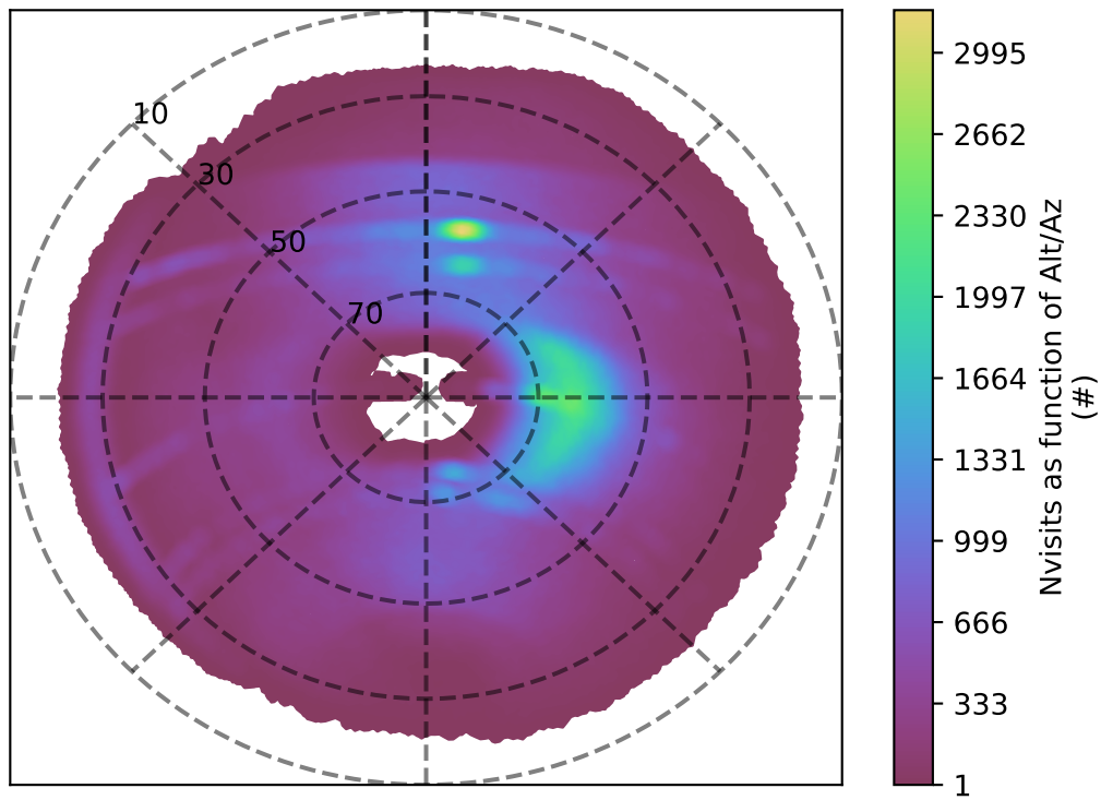
ddf_acor_sf15_lsf30_lsr10_v3.4_10yrs r band: Nvisits as function of Alt/Az
