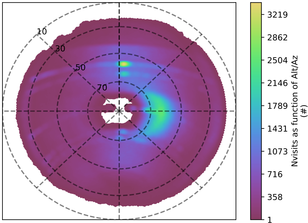
ddf_acor_sf15_lsf30_lsr10_v3.4_10yrs i band: Nvisits as function of Alt/Az
