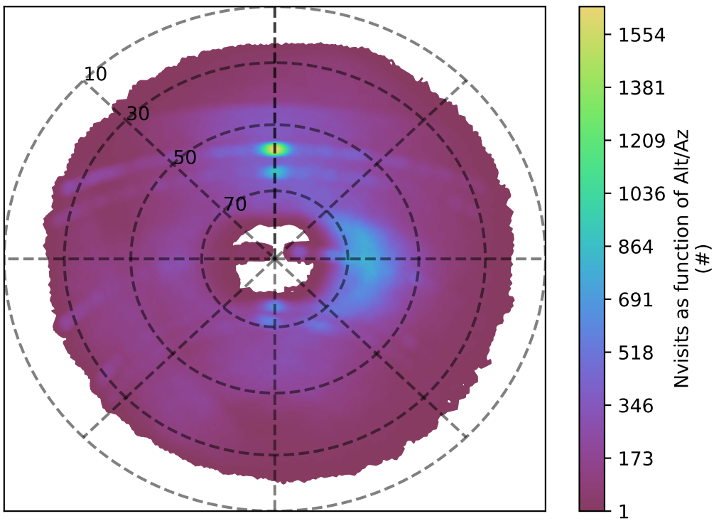
ddf_acor_sf15_lsf30_lsr10_v3.4_10yrs g band: Nvisits as function of Alt/Az
