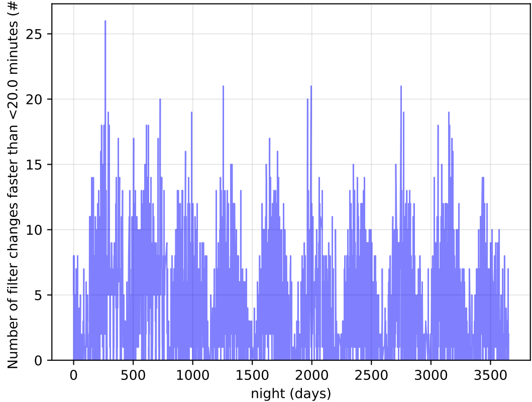
ddf_acor_sf15_Isf30_Isr10_v3.4_10yrs Per Night: Number of filter changes faster than <20.0 minutes
