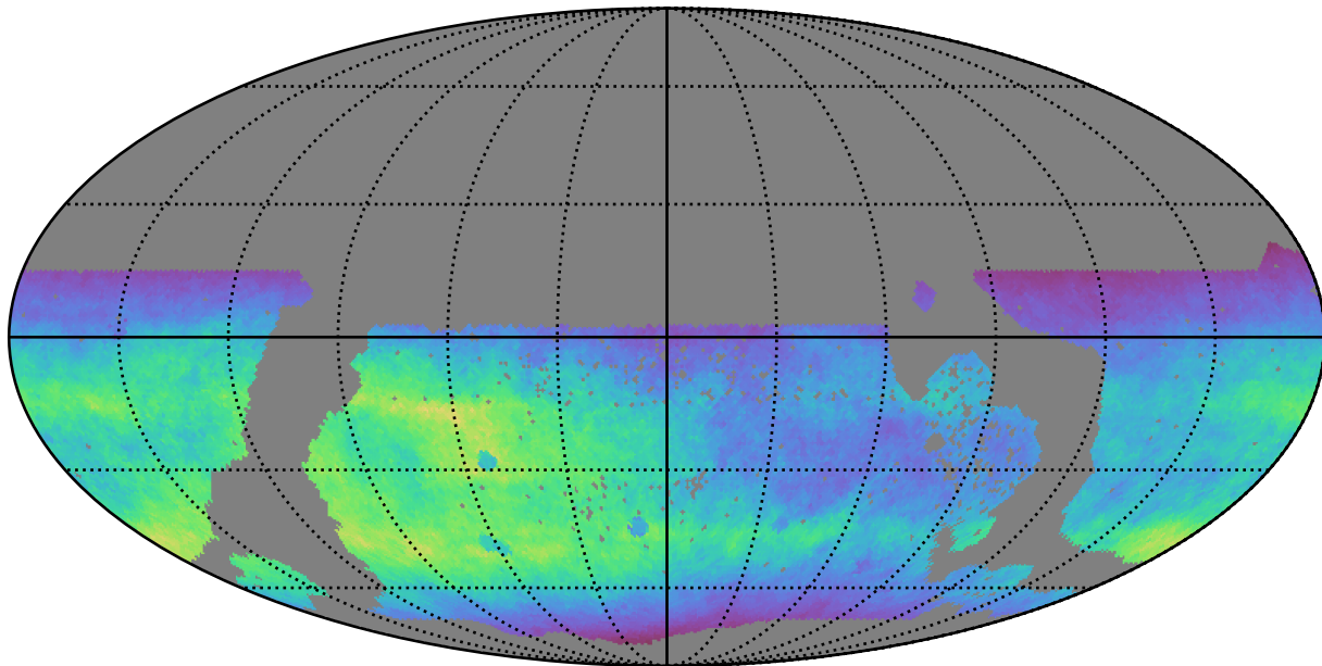
ddf_acor_sf15_lsf30_lsr10_v3.4_10yrs WFD r band: Normalized Teff
