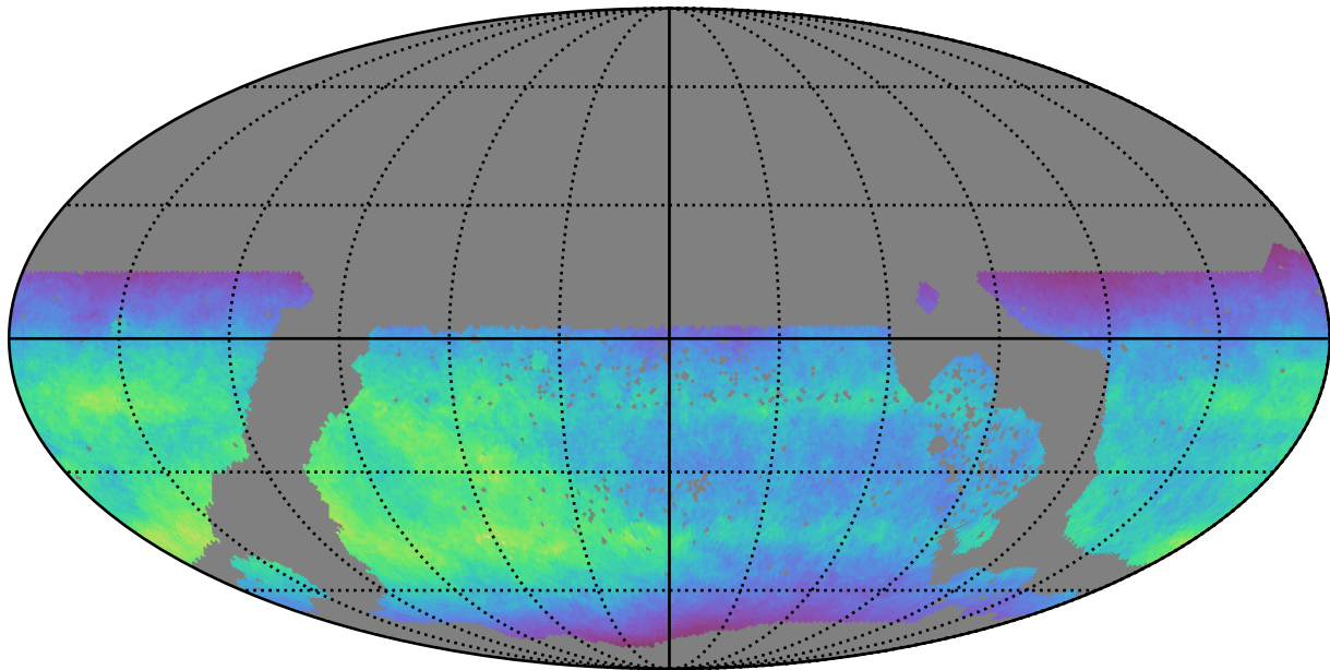
ddf_acor_sf15_lsf30_lsr10_v3.4_10yrs WFD i band: Normalized Teff
