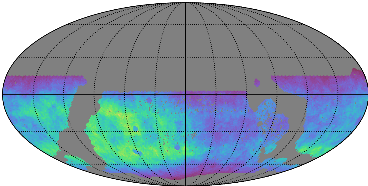
ddf_acor_sf15_lsf30_lsr10_v3.4_10yrs WFD g band: Normalized Teff
