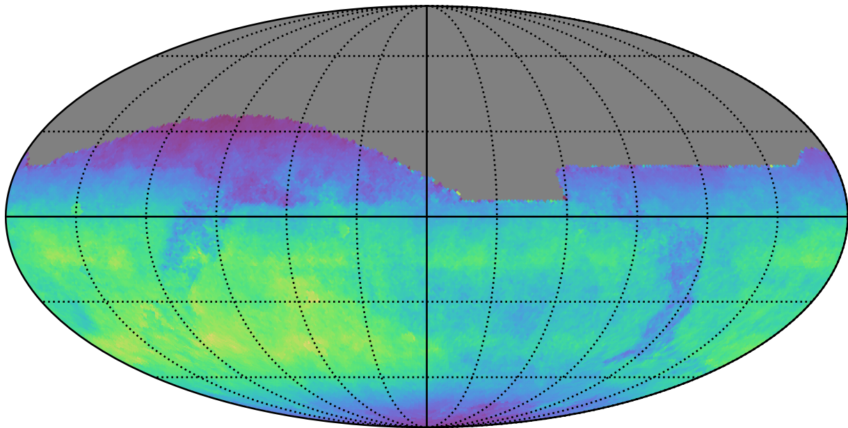
ddf_acor_sf15_lsf30_lsr10_v3.4_10yrs All sky z band: Normalized Teff
