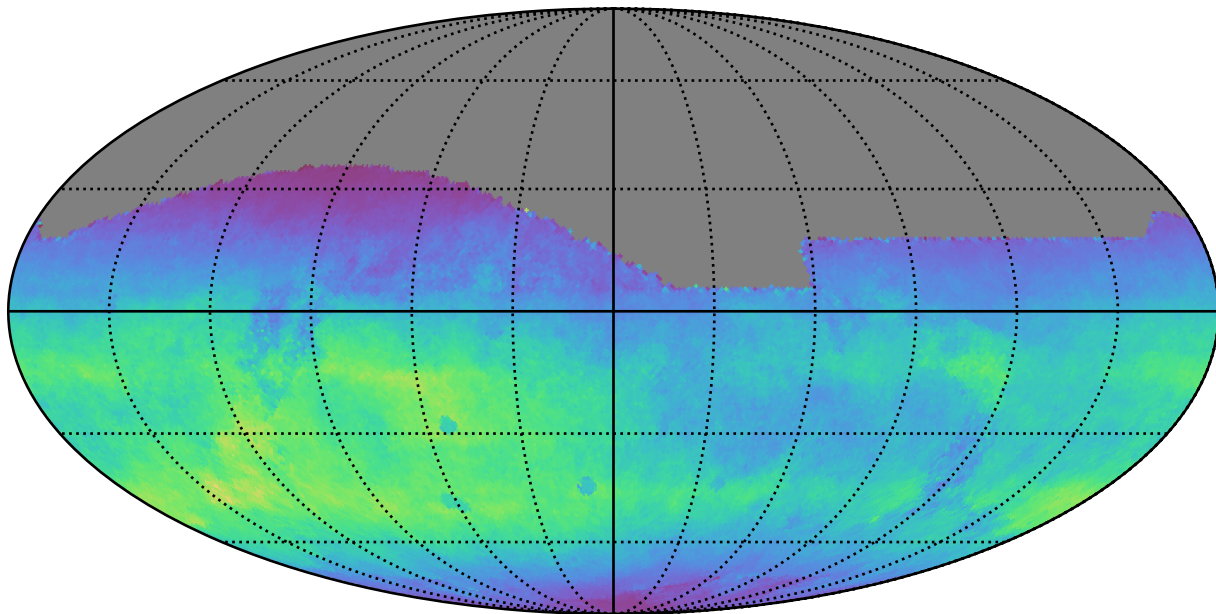
ddf_acor_sf15_lsf30_lsr10_v3.4_10yrs All sky r band: Normalized Teff
