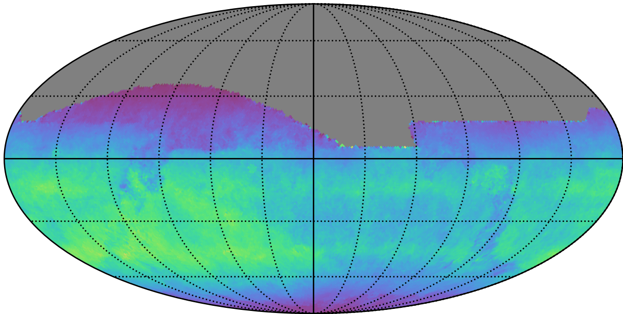
ddf_acor_sf15_lsf30_lsr10_v3.4_10yrs All sky i band: Normalized Teff
