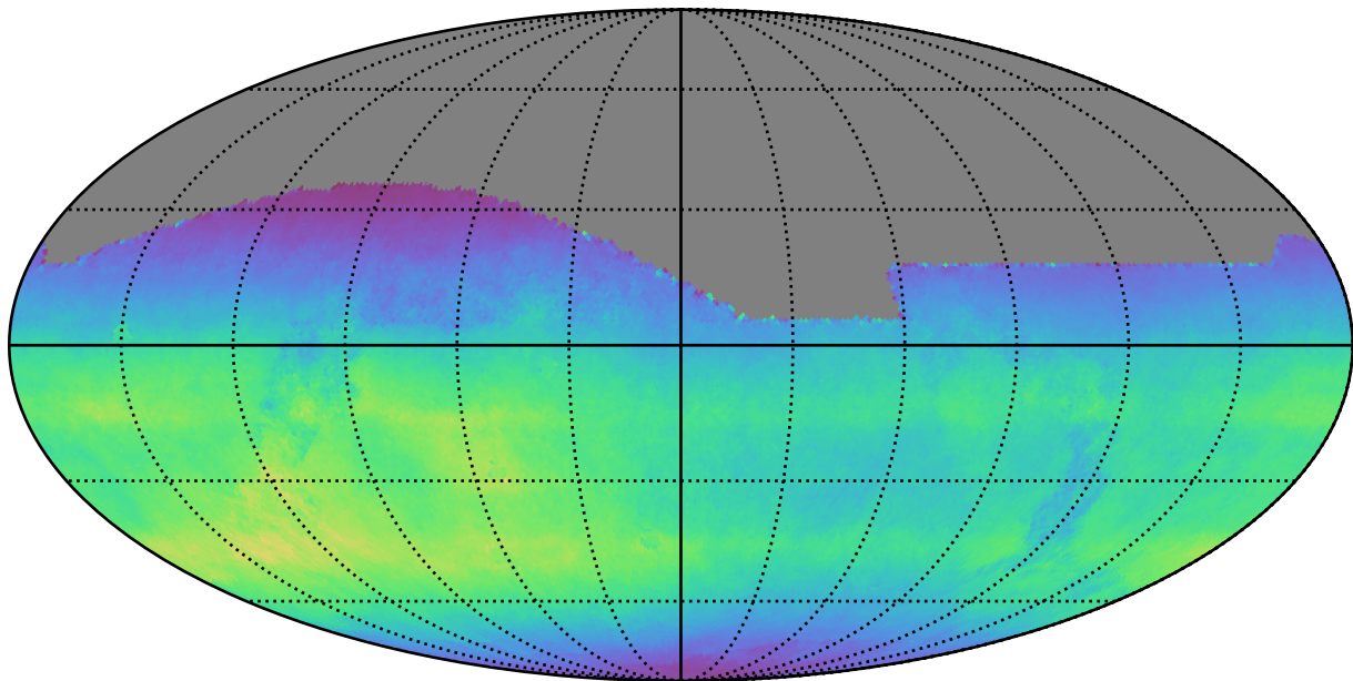
ddf_acor_sf15_lsf30_lsr10_v3.4_10yrs All sky all bands: Normalized Teff
