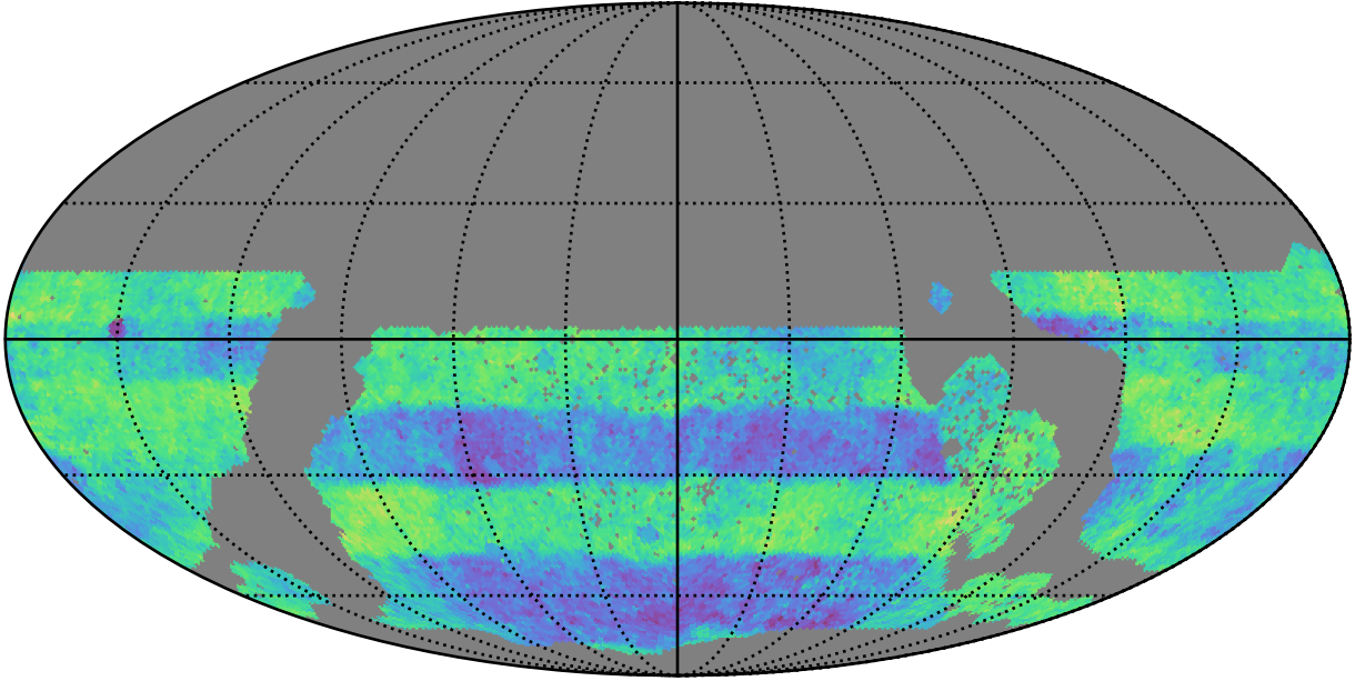
ddf_acor_sf15_lsf30_lsr10_v3.4_10yrs WFD: Normalized Proper Motion Uncert @ 24.0
