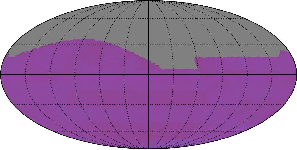
ddf_acor_sf15_lsf30_lsr10_v3.4_10yrs All sky: Normalized Proper Motion Uncert @ 24.0
