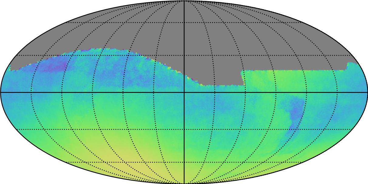
ddf_acor_sf15_lsf30_lsr10_v3.4_10yrs All sky: Normalized Parallax Uncert @ 22.4
