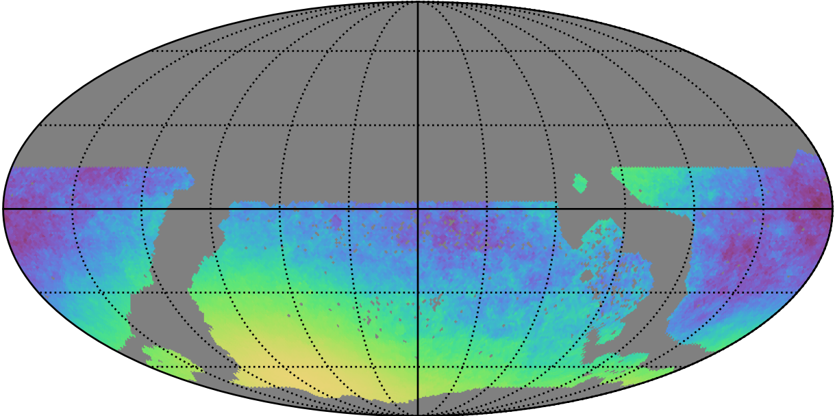
ddf_acor_sf15_lsf30_lsr10_v3.4_10yrs WFD y band only: Normalized Parallax Uncert @ 21.3
