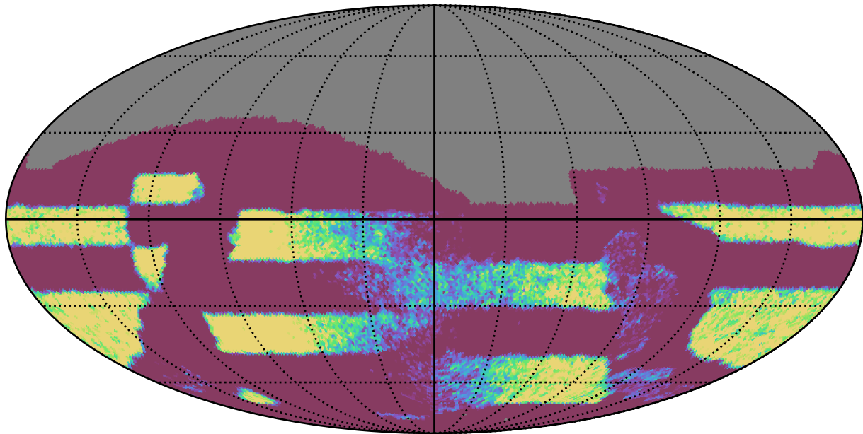
ddf_acor_sf15_lsf30_lsr10_v3.4_10yrs Yr 3-4 all bands: NVisits
