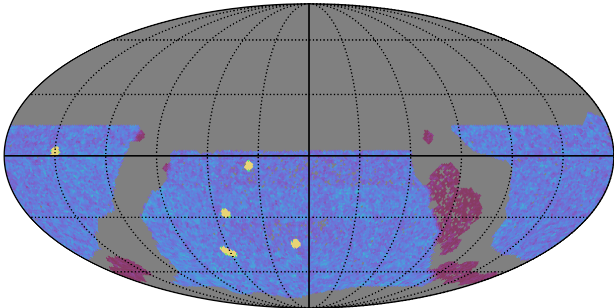
ddf_acor_sf15_lsf30_lsr10_v3.4_10yrs WFD y band: NVisits
