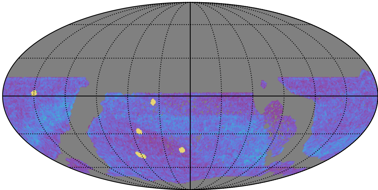
ddf_acor_sf15_lsf30_lsr10_v3.4_10yrs WFD all bands: NVisits
