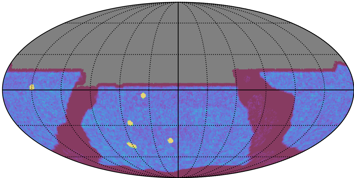
ddf_acor_sf15_lsf30_lsr10_v3.4_10yrs All sky y band: NVisits
