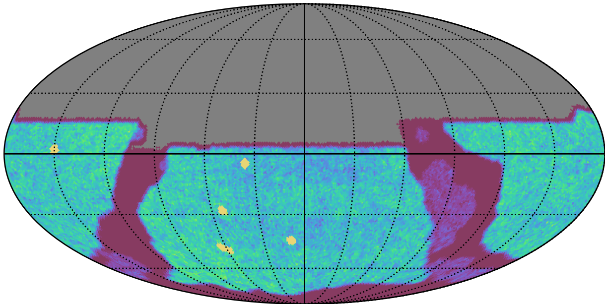
ddf_acor_sf15_lsf30_lsr10_v3.4_10yrs All sky u band: NVisits
