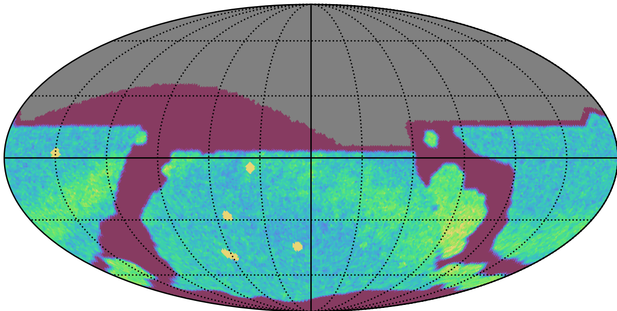
ddf_acor_sf15_lsf30_lsr10_v3.4_10yrs All sky r band: NVisits
