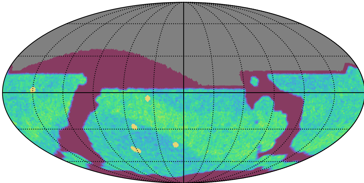
ddf_acor_sf15_lsf30_lsr10_v3.4_10yrs All sky i band: NVisits
