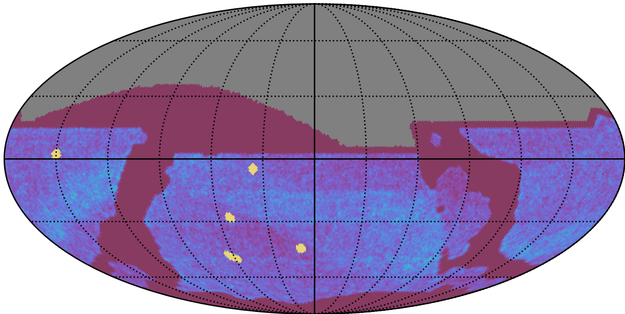
ddf_acor_sf15_lsf30_lsr10_v3.4_10yrs All sky all bands: NVisits
