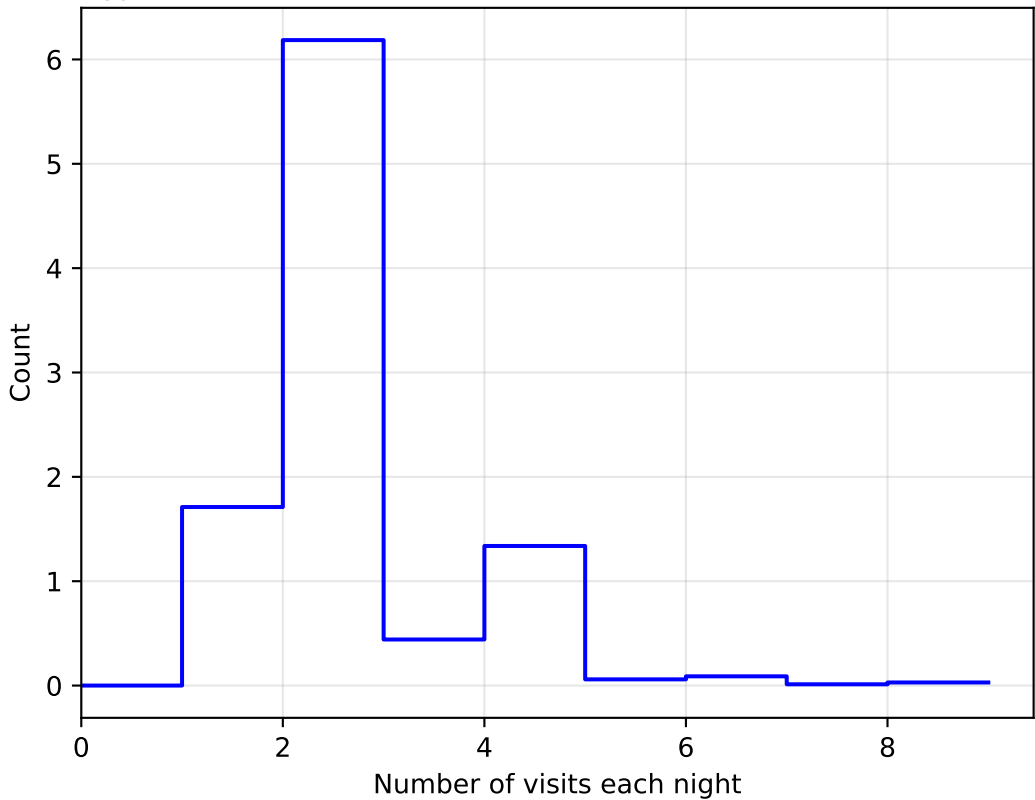
ddf_acor_sf15_lsf30_lsr10_v3.4_10yrs All sky: NVisitsPerNight 1e6
