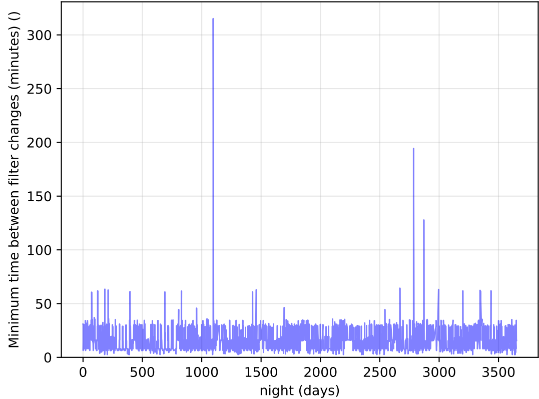
ddf_acor_sf15_Isf30_Isr10_v3.4_10yrs Per Night: Minimum time between filter changes (minutes)
