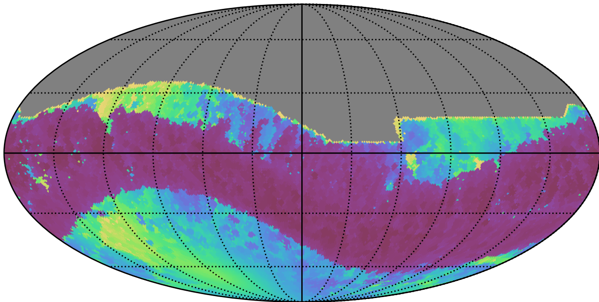
ddf_acor_sf15_lsf30_lsr10_v3.4_10yrs All sky i band: Min solarElong
