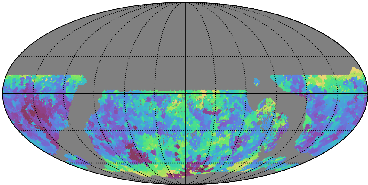
ddf_acor_sf15_lsf30_lsr10_v3.4_10yrs WFD u band: Min seeingEff
