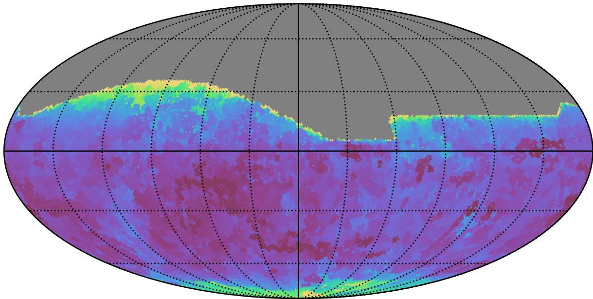
ddf_acor_sf15_lsf30_lsr10_v3.4_10yrs All sky r band: Min seeingEff
