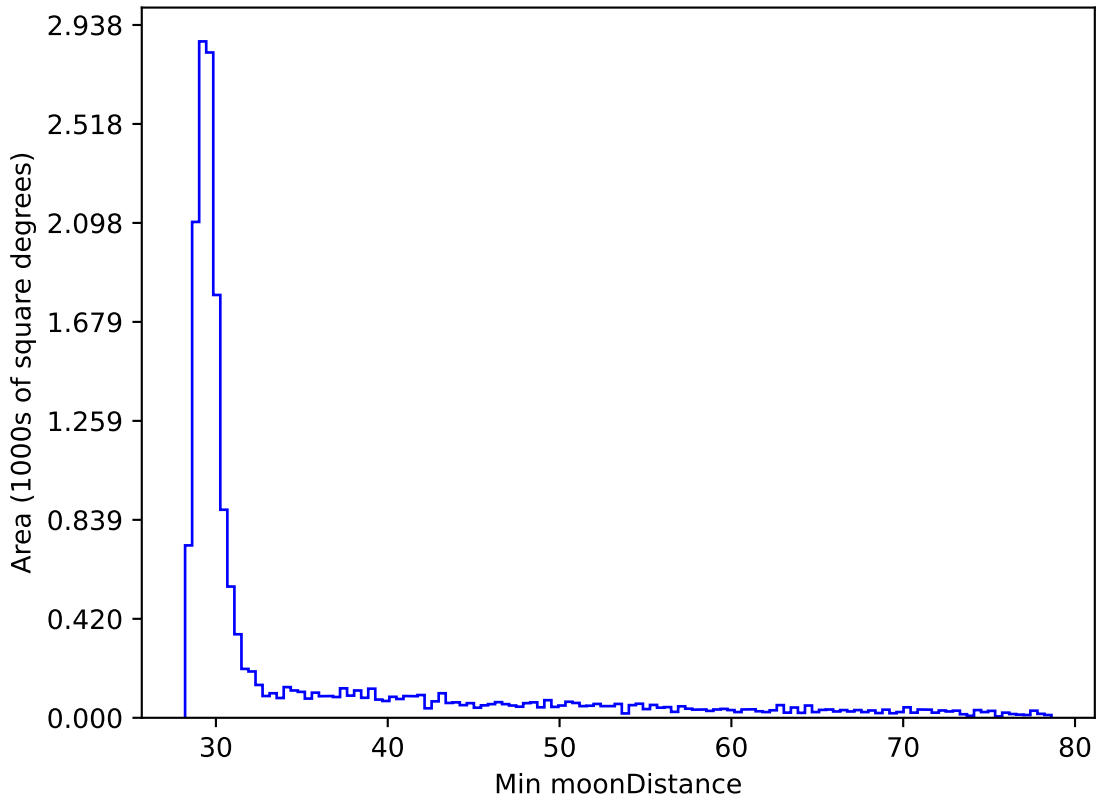
ddf_acor_sf15_lsf30_lsr10_v3.4_10yrs WFD y band: Min moonDistance
