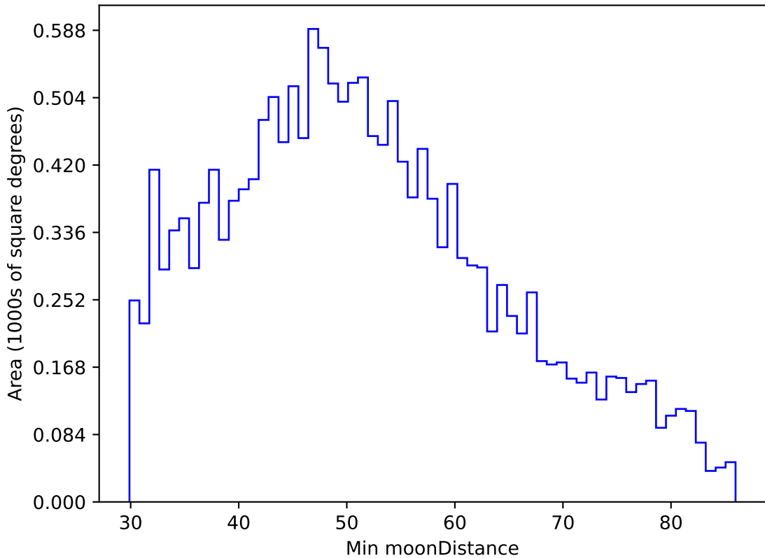
ddf_acor_sf15_lsf30_lsr10_v3.4_10yrs WFD u band: Min moonDistance
