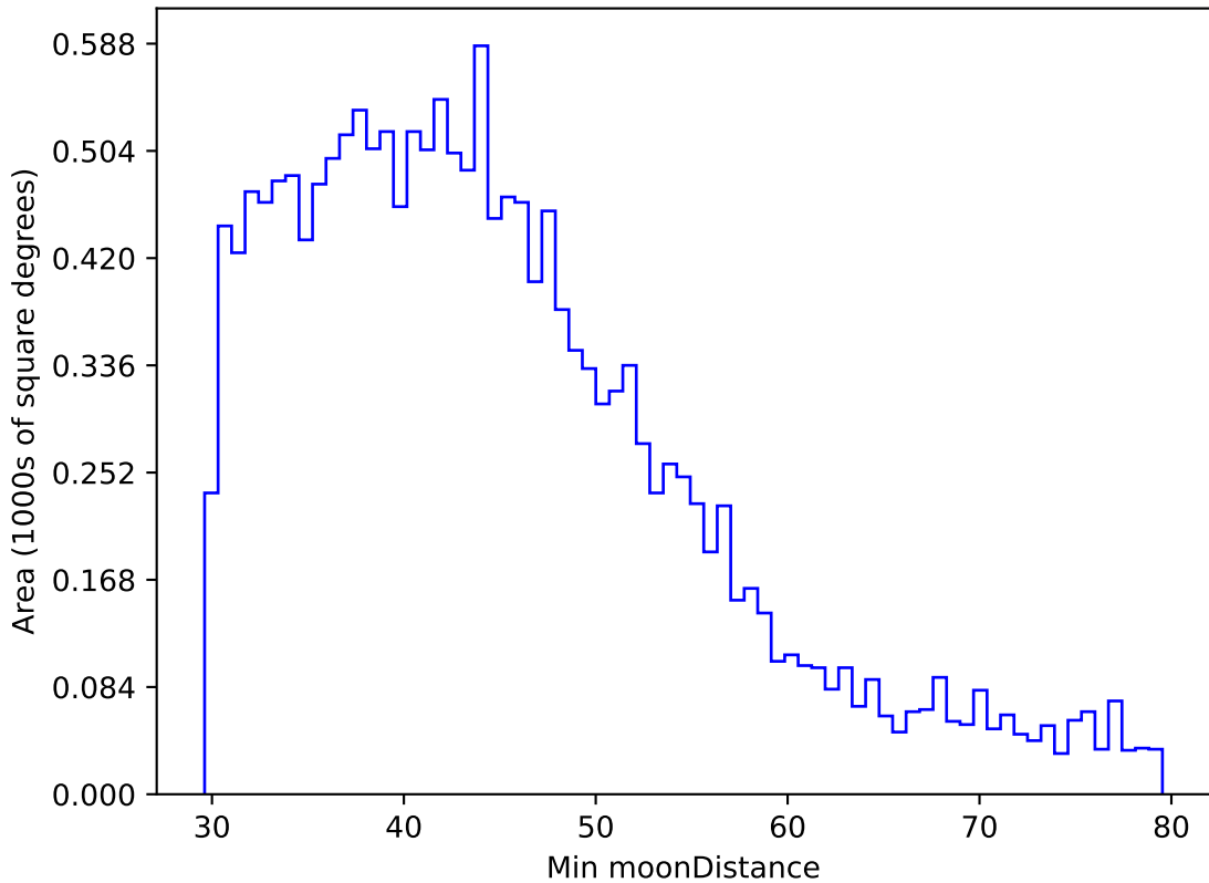
ddf_acor_sf15_lsf30_lsr10_v3.4_10yrs WFD g band: Min moonDistance
