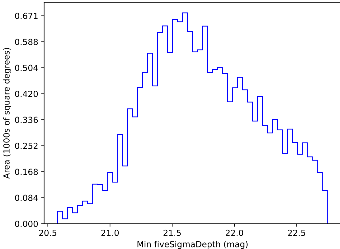
ddf_acor_sf15_lsf30_lsr10_v3.4_10yrs WFD i band: Min fiveSigmaDepth
